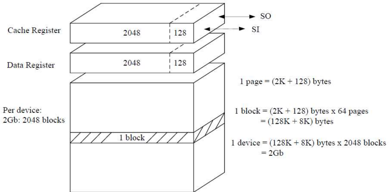
Figure1. Array Organization
