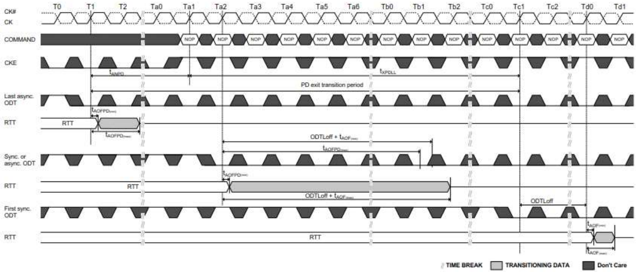
Figure 4-76 Transition period for short CKE cycles, entry and exit period overlapping
