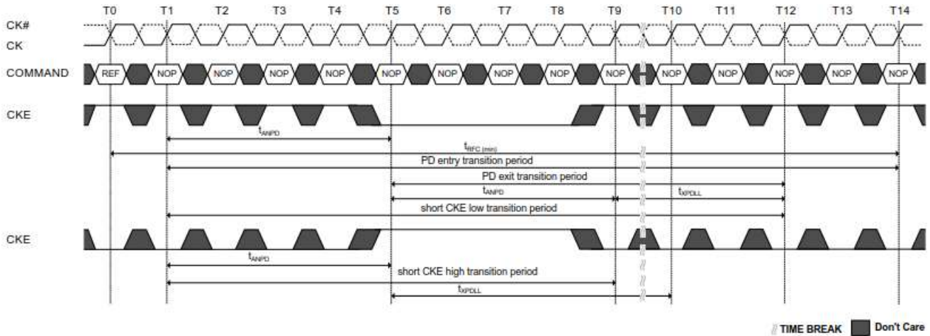
Figure 4-76 Transition period for short CKE cycles, entry and exit period overlapping
