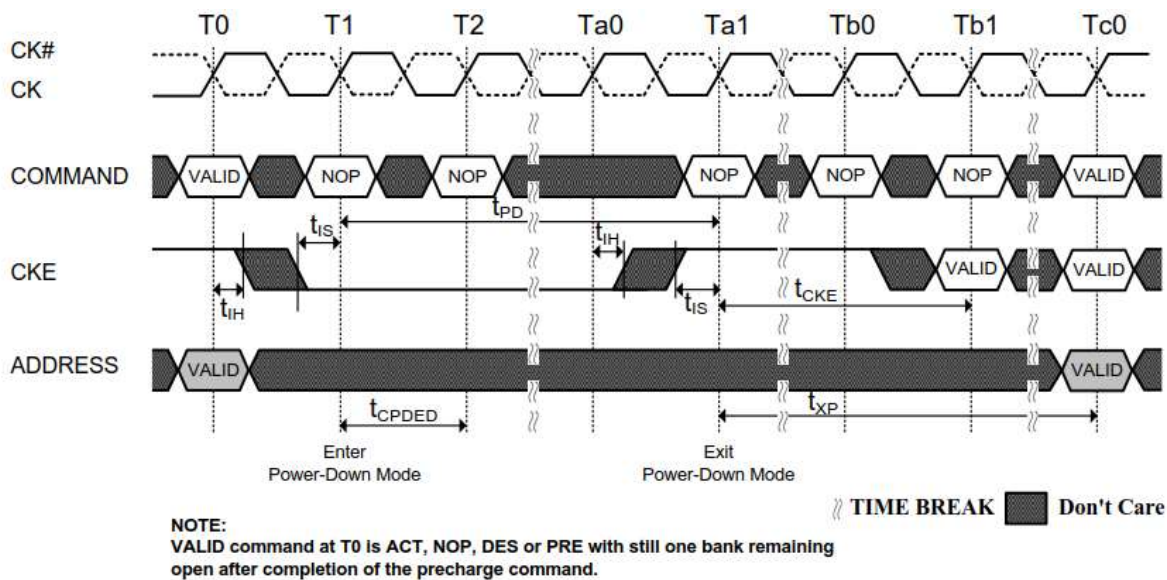
Figure 4-55 Active Power-Down Entry and Exit Timing Diagram
