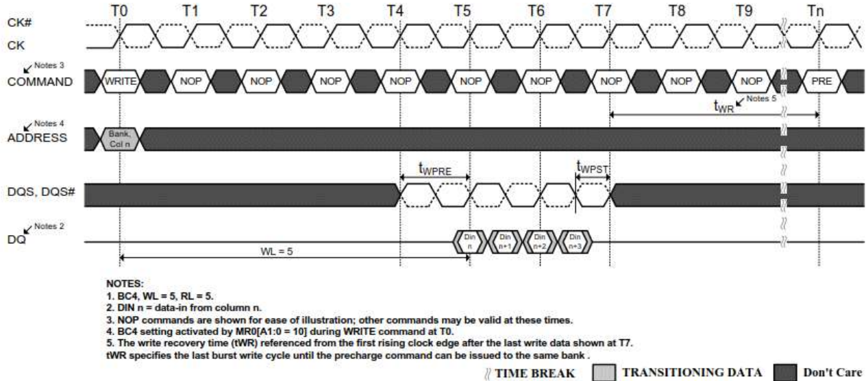
Figure 4-44 WRITE (BC4) to Precharge Operation
