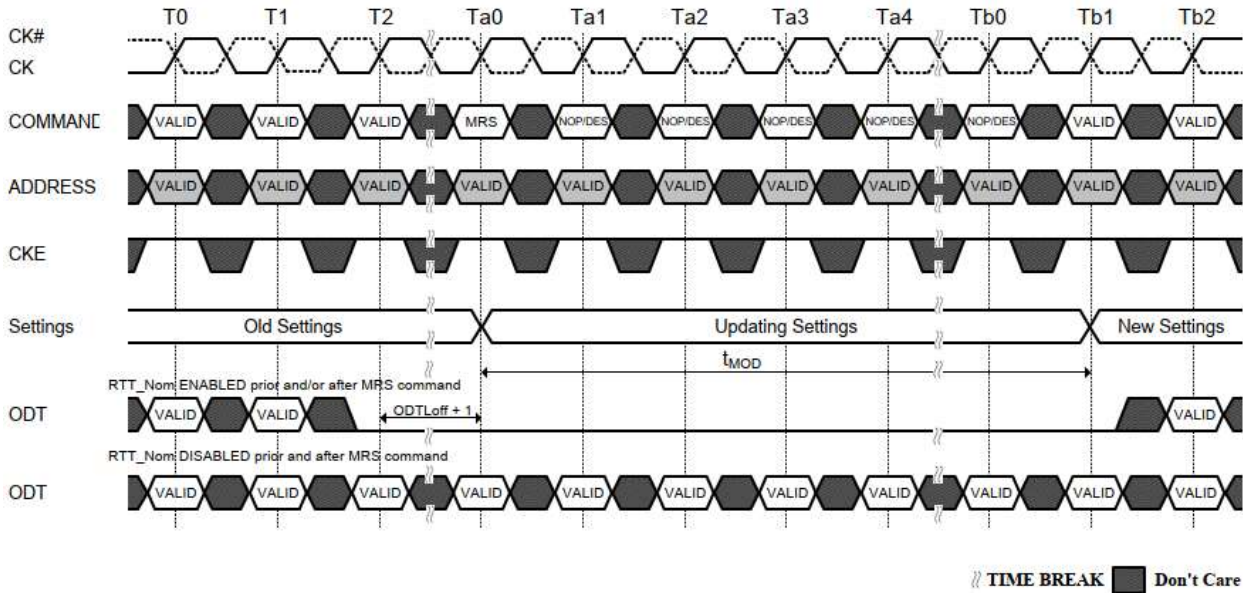
Figure 4-4 tMOD timing
